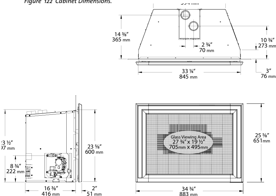
Figure 122 Cabinet Dimensions.
