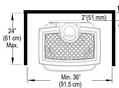
Figure 27. Alcove Installation Clearances.
