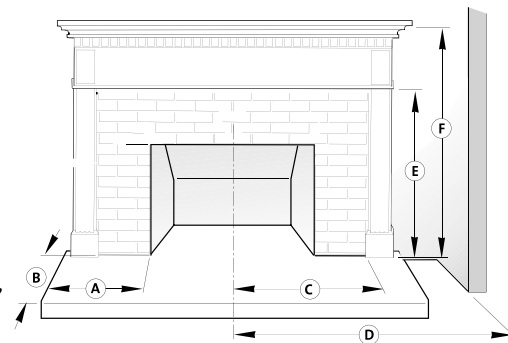
Figure 106. Clearance requirements
