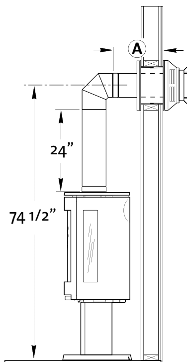
Figure 60. Minimum vent pipe sections required for horizontal termination: A = 12" with NG 18" with LP
