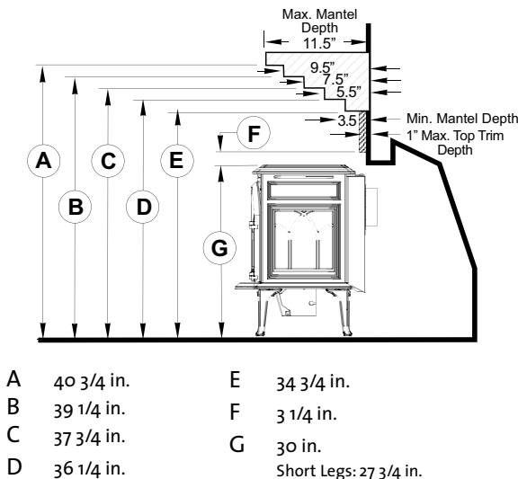
Figure 97. Mantel Clearances - stove flush with fireplace face.
