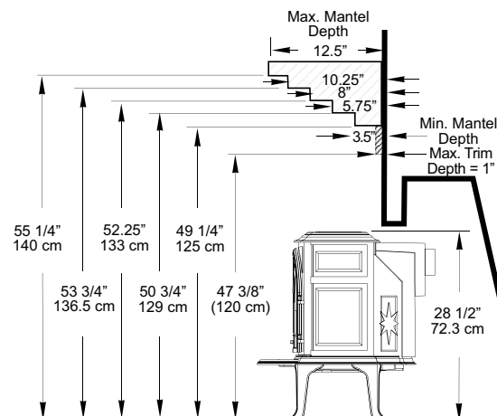
Figure 140 Mantel and Trim specifications - Stove installed with Top Plate flush with fireplace face.
