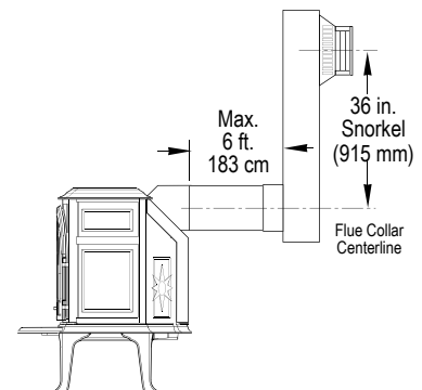
Figure 67. * Maximum Horizontal with 36" Snorkel Termination.
