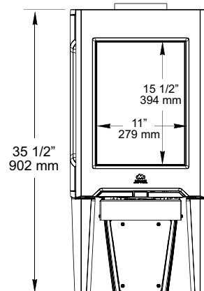
Figure 8. GF 160 DV IPI dimensions
