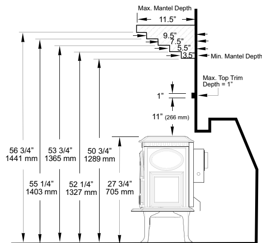
Figure 135. Mantel and Trim specifications - Stove installed with rear shroud flush to fireplace face.
