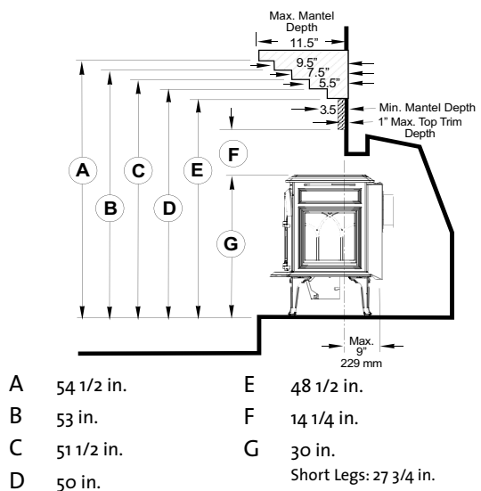
Figure 98. Mantel Clearances - stove recessed into fireplace, 9" max .
