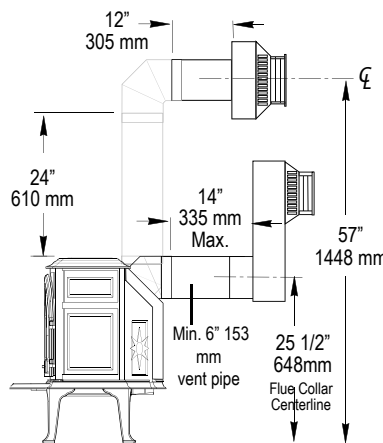
Figure 66. * • Minimum vent for horizontal termination. • 14" Maximum horizontal run directly off rear of stove with 14" Snorkel termination.
