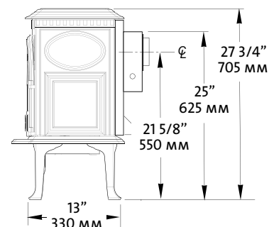
Figure 132 Primary dimensions. With optional Short Legs, reduce height by 2 1/4".
