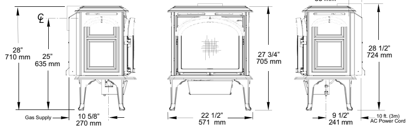
Figure 26. GF 300 DV Allagash Critical Dimensions. Subtract 2 1/4" from height for Short Leg option.
