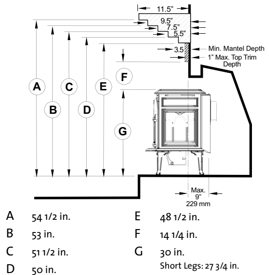
Figure 88. Mantel Clearances - stove recessed into fireplace, 9" max.
