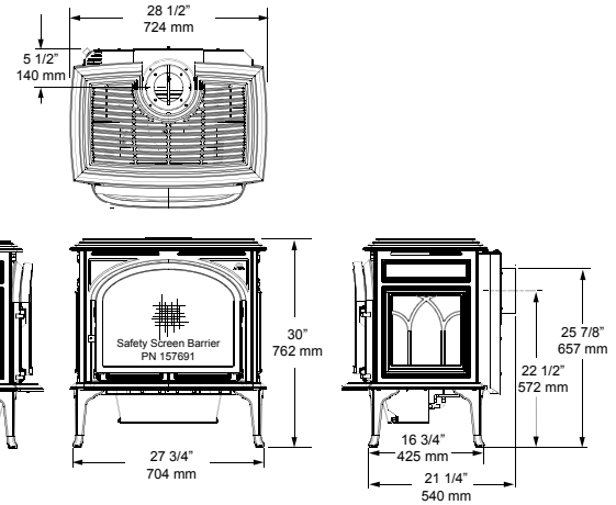
Figure 92. GF 500 DV Portland dimensions.
