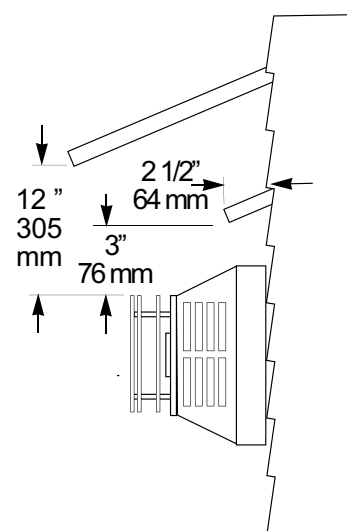
Figure 7. Vent Terminal Clearances - Overhangs
