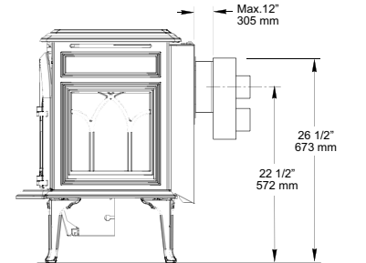
Figure 94. GF 500 DV Rear Exit Centerline with Co-linear Adaptor
