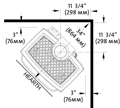
Figure 134 Vent adaptor centerline at minimum clearance to corner walls.
