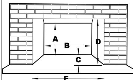
Figure 116. Fireplace dimensions
