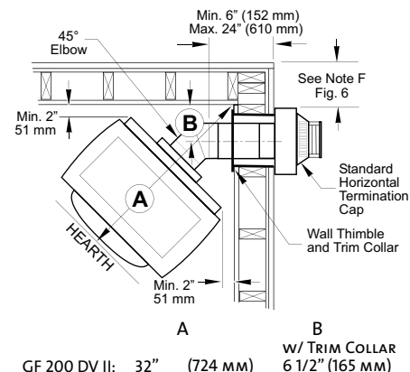
Figure 20. GF 200 DV II Corner with 45° elbow.
