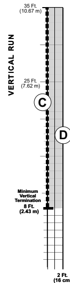
Figure 71. Colinear Termination / LP.
