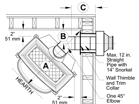
Figure 68. Corner Installation at min. clearance with Snorkel Termination.
