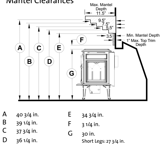
Figure 87. Mantel Clearances - stove flush with fireplace face.
