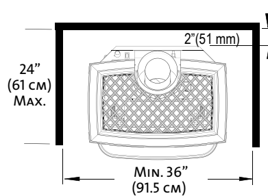
Figure 40. Alcove Installation Clearances.
