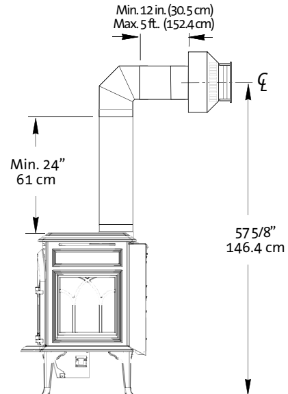
Figure 100. Min./Max. vent required for horizontal termination.
