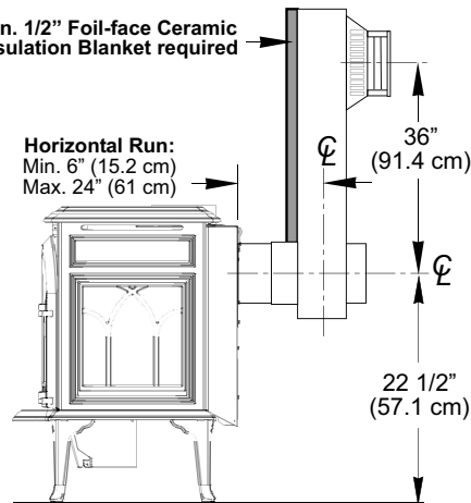
Figure 99. Min./Max. horizontal and vertical vent run 36" Snorkel termination.
