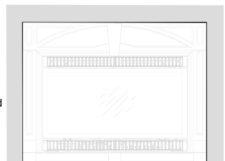
Figure 105. Wide Surround Assembly
