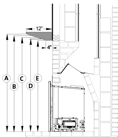
Figure 113. Mantel and ceiling clearances
