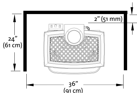
Figure 133 Alcove Installation Clearances.
