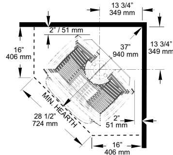
Figure 85. Corner Installation clearances and minimum hearth pad.
