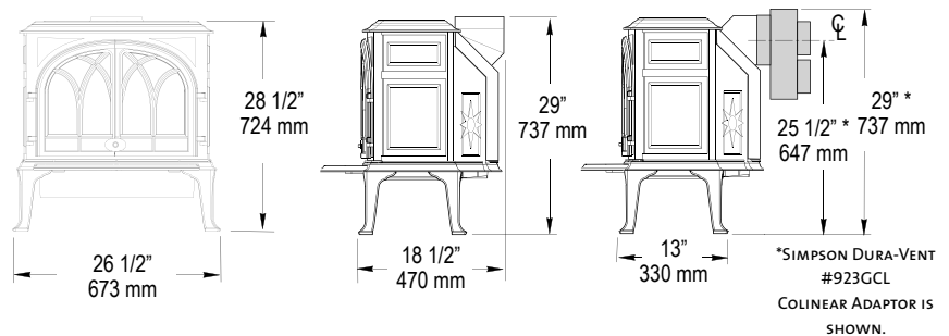
Figure 63. GF 400 DV Sebago dimensions. Subtract 2 1/4" from height for Short Leg option.
