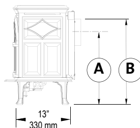
Figure 22 GF 200 DV II Rear Exit Centerlines and Collar Height
