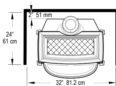
Figure 64. Alcove Installation Clearances.
