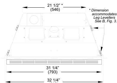
Figure 102. GI 450 DV Katahdin dimensions.
